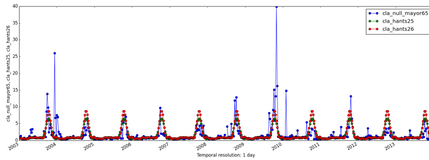
(b) PMN
