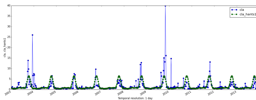
(a) NOF = 5
