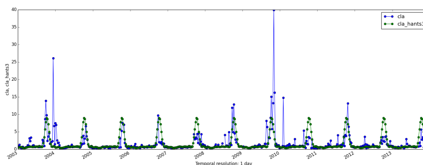
(c) NOF = 7
