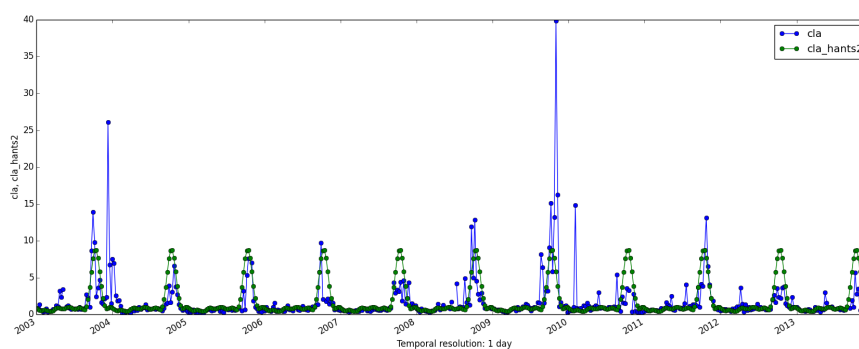
(b) NOF = 6
